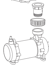
Fig. 22 Pump Assembly
