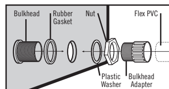
Bulkhead assembly.
