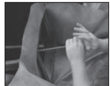
Fig. 16 Replace the skimmer liner plate and the two corner screws, and then proceed with the bottom two corners. Punch remaining holes, thread screws.
